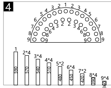
Glass column installation diagram
