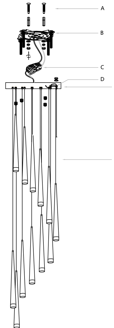
Lamp cap suspension wire installation diagram: The shortest one is 1, and the longest one is 12.
